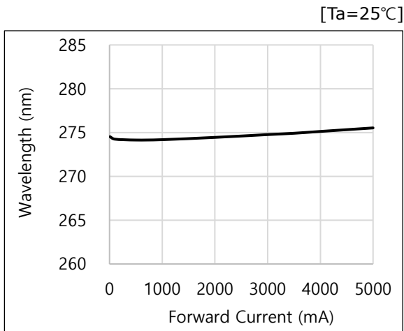
3) Peak Wavelength vs. Forward Current
